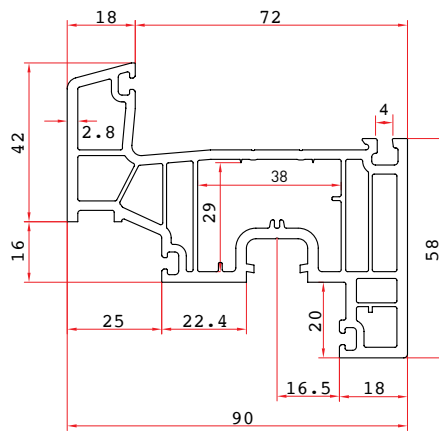
Sash Profile
