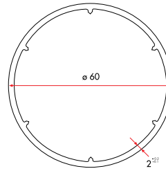
Pipe Profile
