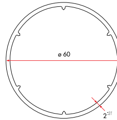
Pipe Profile
