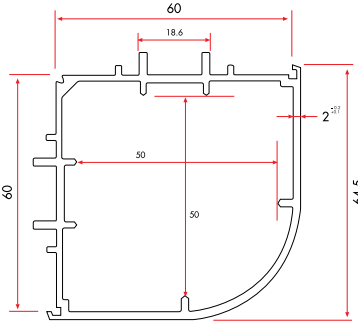
90° Corner Adaptor
