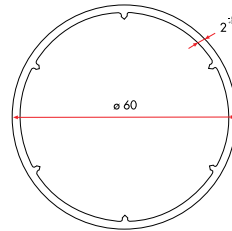
Pipe Profile
