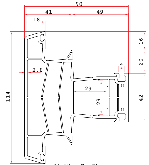
Mullion Profile
