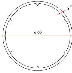
Pipe Profile
